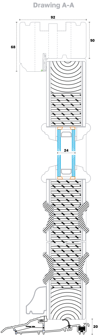
Doorset with 54mm SBD Composite Door
